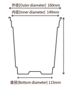
⑤ 双色花盆(Double Color Pot) 160x140mm
