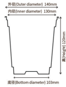
⑦ 双色花盆(Double Color Pot) 140x120mm
