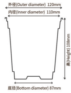
⑨ 双色花盆(Double Color Pot) 120x108mm
