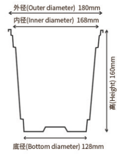
③ 双色花盆(Double Color Pot) 180x160mm
